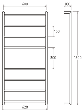
TLH6-130x60
