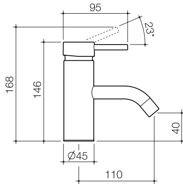
Liano Nexus Basin Mixer WELS 6 star rated, 4.5L/min 96193B6A
