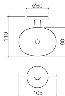
Liano Nexus Soap Dish 96126B
