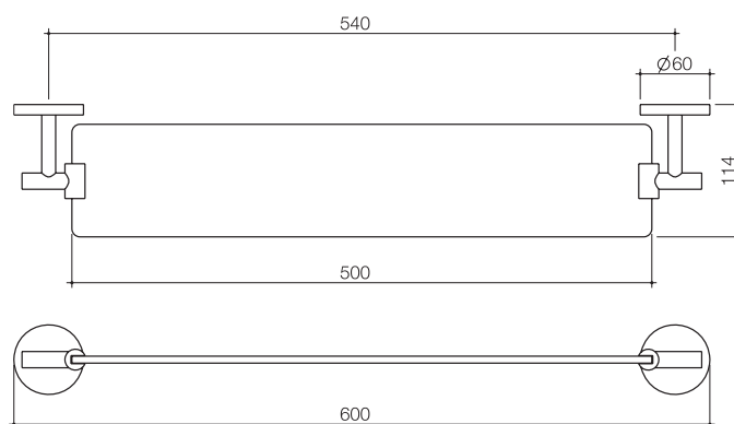
Liano Nexus Glass Shelf 96127B
