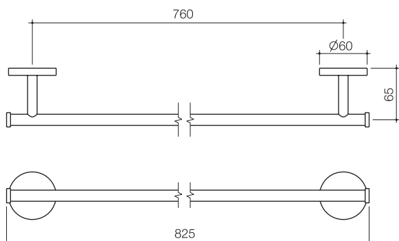
Liano Nexus Single Towel Rail 96120B
