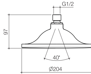
Liano Nexus Overhead Rain Shower Head WELS 2 star rated, 12L/min 91051B2A
