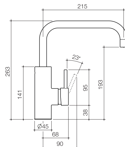
Liano Nexus Sink Mixer WELS 5 star rated, 6L/min 96194B5A
