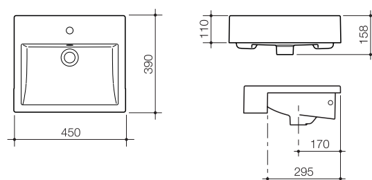
Liano Nexus Semi-Recessed Basin
