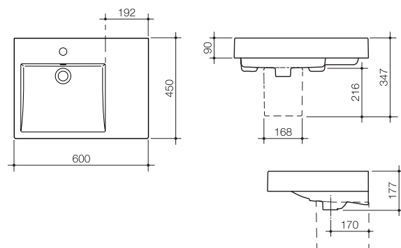
Liano Nexus 600 Wall Basin Right Hand Shelf
