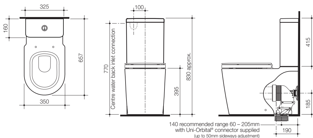
Liano Wall Faced Close Coupled BE Toilet Suite
