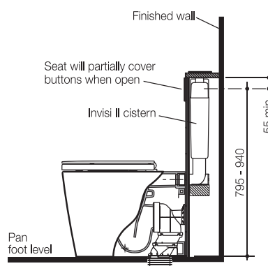
Under Counter Installation
