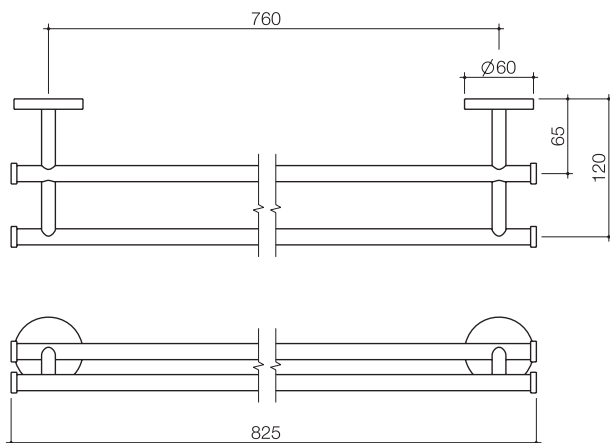
Liano Nexus Double Towel Rail 96121B
