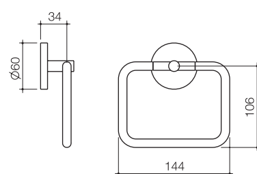
Liano Nexus Hand Towel Ring 96122B
