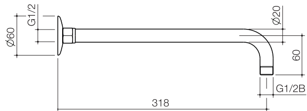
Liano Nexus Right Angle Shower Arm 2464.04B
